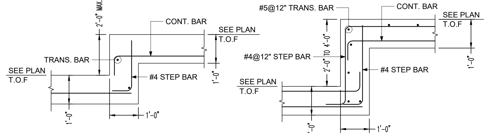
TYP. FOOTING STEP DETAIL Scale - 1/2"=1'-0" REF: 7.12/S5.1
